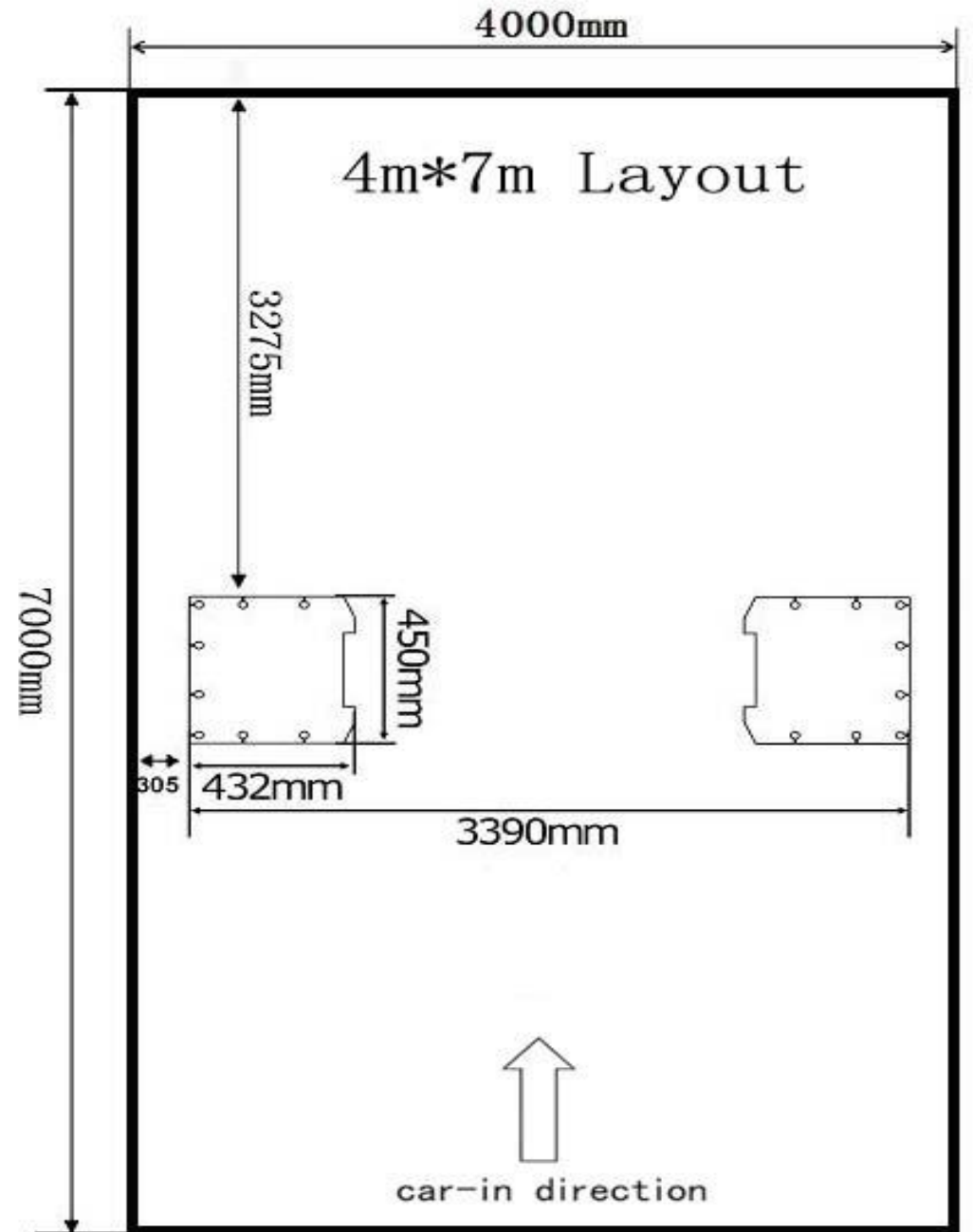
Classic BP4 Concrete Drawing
