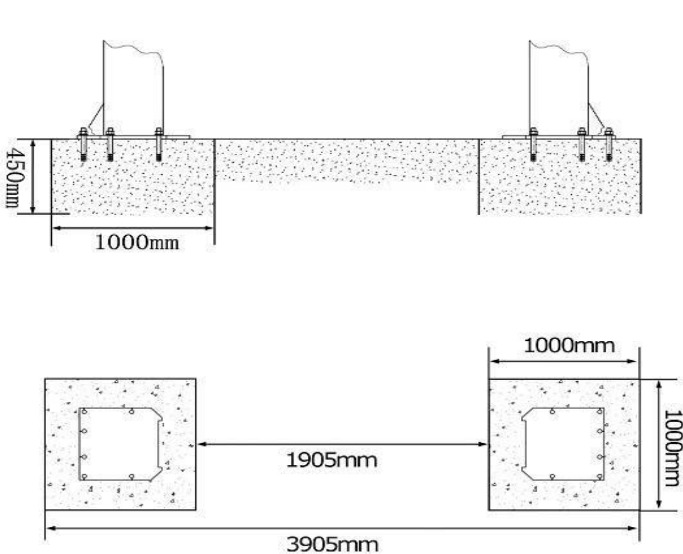
Classic BP4-L Concrete Drawing
