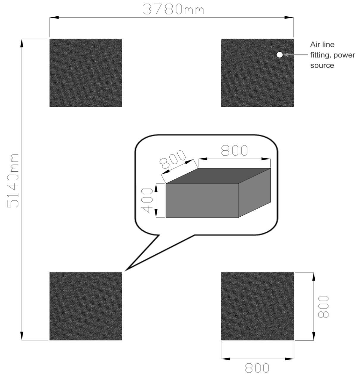
Classic CL4000-4P Concrete Drawing
