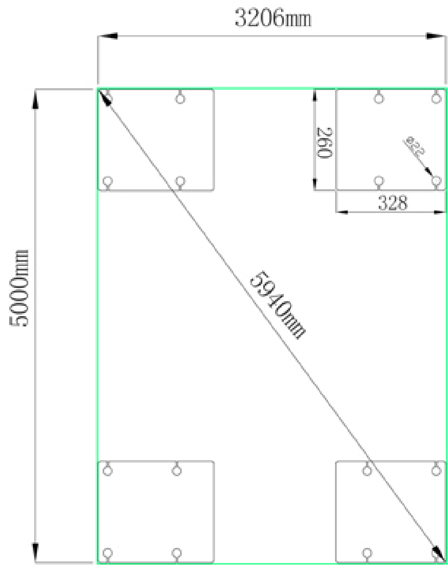
Classic CL4000HP Concrete Drawing
