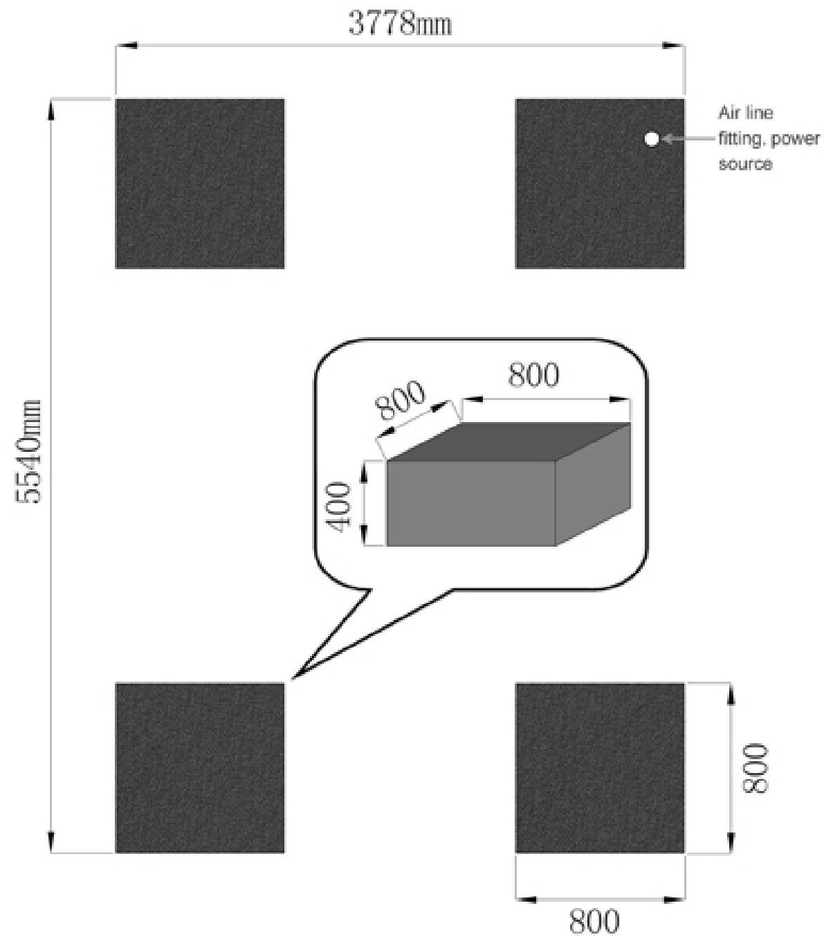
Classic CL4000HP Concrete Drawing
